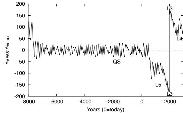
Figure 2. The mean longitude difference of 2002 VE68 and Venus.
